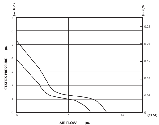
Performance Curve
